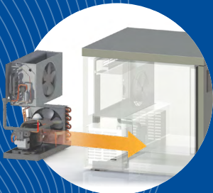
Back Mount
